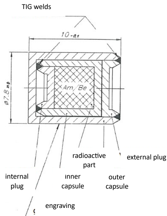
Figure 1: SFRM of the construction type Am1.N02. The illustration corresponds to the technical drawing "Am Be Neutronenquelle, Am1.N02, 1.207.02.02-00:00(4), BEBIG Isotopentechnik und Umweltdiagnostik GmbH" of 9 May 1995.
